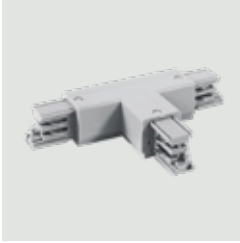
Dimensions Description Color Color L: 17cm W: 10cm H: 3.4cm T Connector for 3 Circuit Lighting Track 100-240V Black / Code 19408 White / Code 19409
