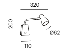
KID. AP-1453 1x GU10 LED - 7W 3000K | 600lm OX Antique gold IP20 CE 230V | 50Hz
