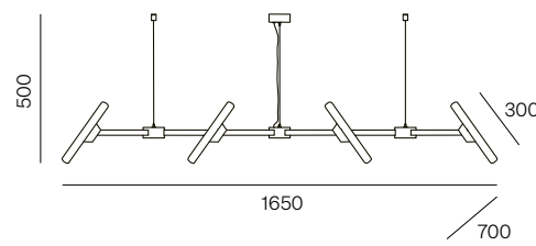
OKKU. SU-0992 💡 8x S14D MAX. 8W LED ☐ IP20 ☐ CE 230V | 50Hz
