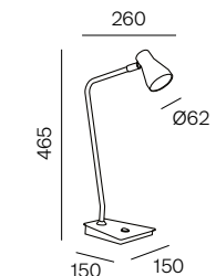
KID. CM-0537 1x GU10 LED - 7W 3000K | 600lm OX Antique gold IP20 CE 230V | 50Hz
