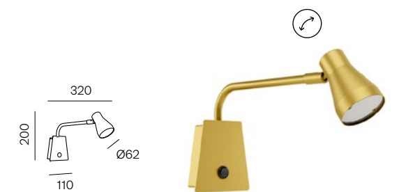
KID. AP-1453 1x GU10 LED - 7W 3000K | 600lm OX Antique gold IP20 CE 230V | 50Hz
