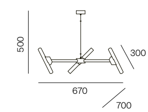
OKKU. SU-1007 💡 3x S14D MAX. 8W LED ☐ IP20 ☐ CE 230V | 50Hz
