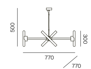
OKKU. SU-1009 💡 4x S14D MAX. 8W LED ☐ IP20 ☐ CE 230V | 50Hz
